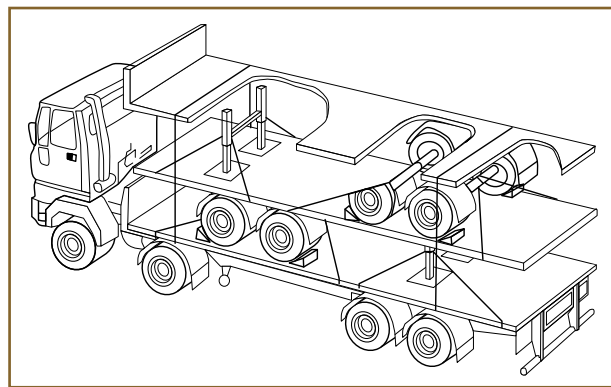
Fig. 71. Trailers loaded on a trailer
