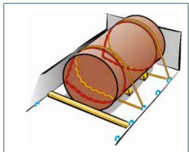
Fig. 25. Loop lashing combined with base blocking
