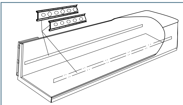
Fig. 43. Attaching rails
